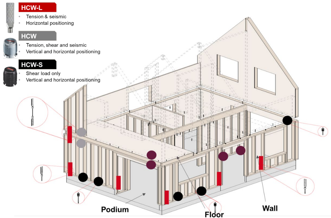
Fig. 2.1: The Hilti Coupler Wood is available in three different versions (HCW-L, HCW and HCW-S)
