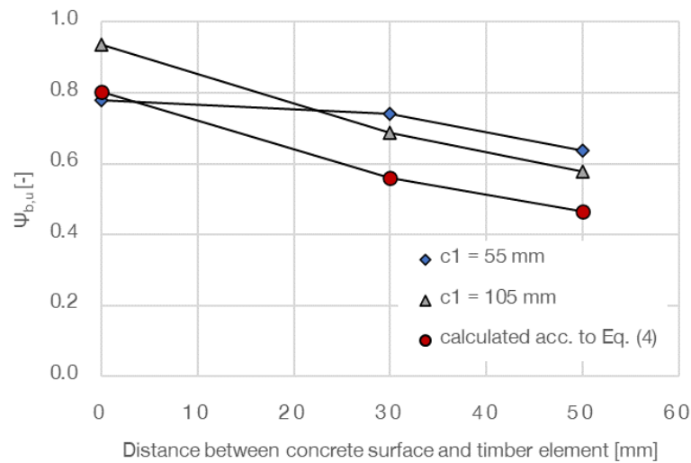
Fig. 4.4: Reduction of failure load with increasing lever arm (right)
