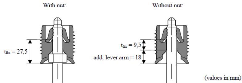
Fig. 3.2: Definition of t_{nx} in case of a levelling nut and t_{nx} and the additional lever arm in case of no levelling nut
