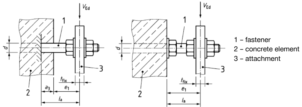
Fig. 4.1: Definition of the lever arm according to EN 1992-4
