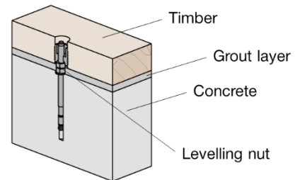
Fig. 2.6: Positioning of the HCW on top of the post-installed anchor with a levelling nut
