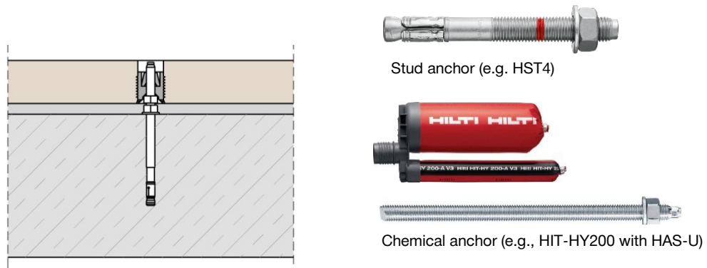
Fig. 2.3: Connection between a timber element and a concrete member with HCW and post-installed anchors
