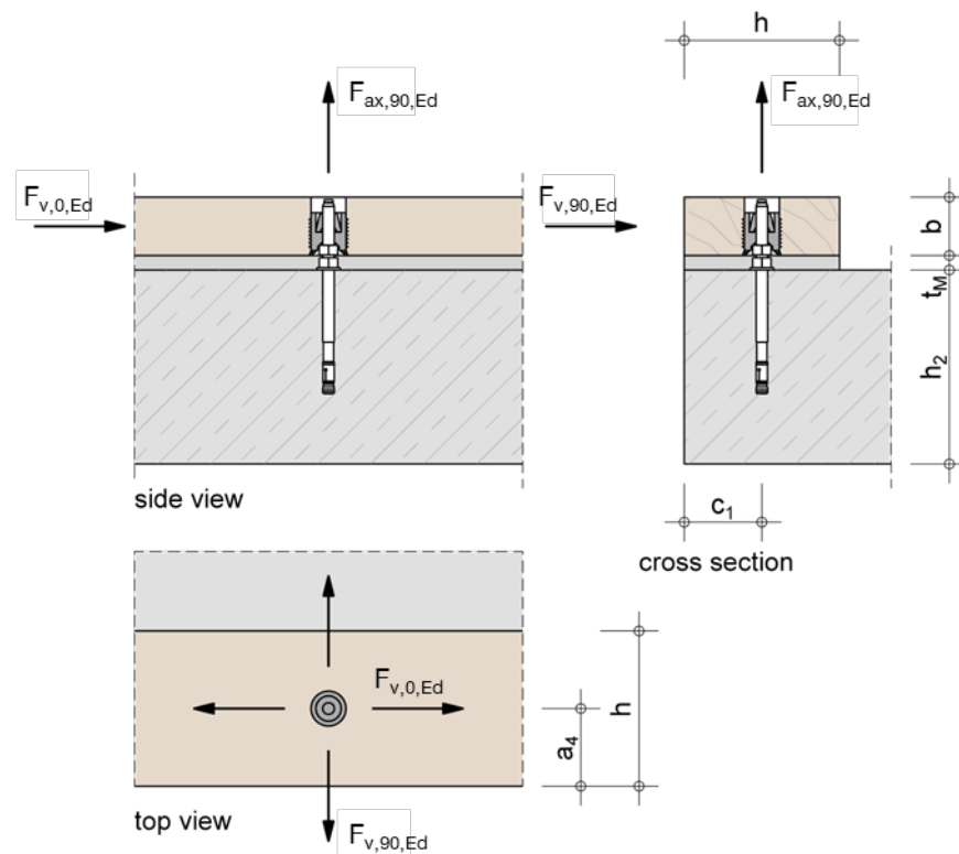
Fig. 6.1: Connection and geometry for the connections
