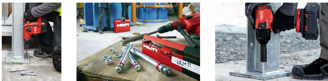
Fig. 8.9: Installation of mechanical anchors using setting tools and impact wrenches
