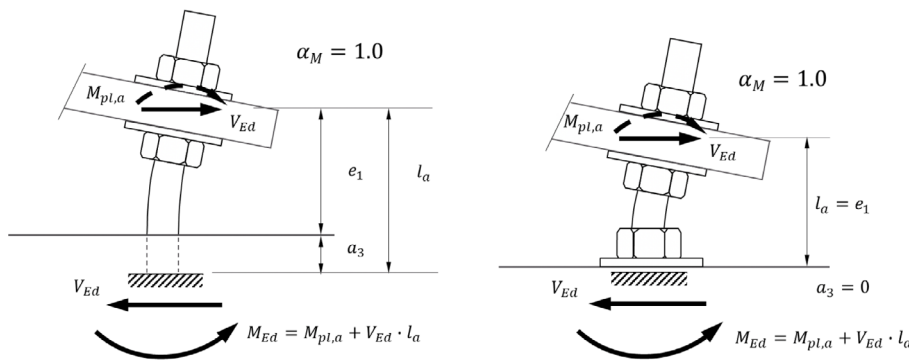
a) Unrestrained rotation of the baseplate (EC2-4 and SOFA)
