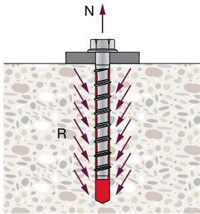
Fig. 3.9: Bonded screw anchor
