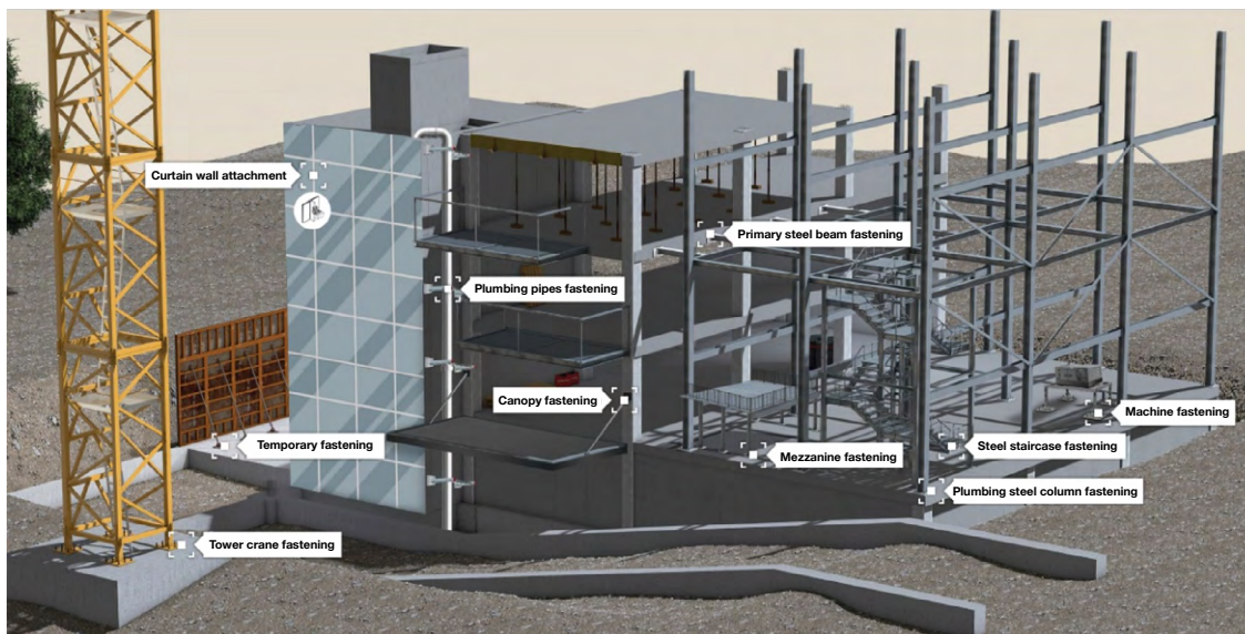
Fig. 2.1: Illustration of typical applications in a building under construction
