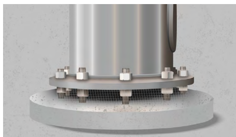
a) Ungrouted stand-off connection: in service
