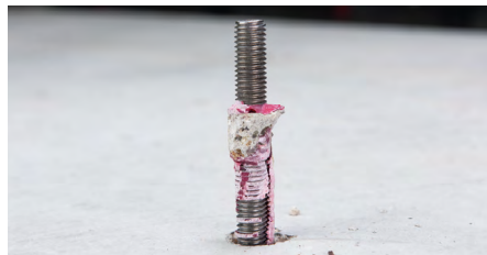
Fig. 3.18: Combined pull-out and concrete cone failure under tension loading
