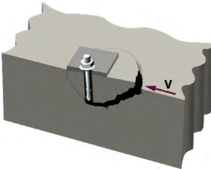
Fig. 3.22: Concrete pry-out failure under shear loading
