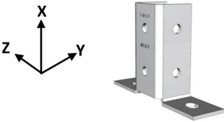
Figure C27: Definition of Hilti MT-B-T, MT-B-T OC, MT-B-T FL and MT-B-T FL OC baseplate local coordinate System for use with Hilti MT-50 S, MT-50, MT-50 U, MT-50 S OC and MT-50 OC installation channels
