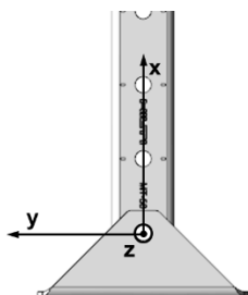
Figure C26: Definition of Hilti MT-AB A set and MT-AB A OC set local coordinate System for use with Hilti MT-50 S, MT-50, MT-50 S OC and MT-50 OC installation channels
