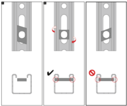
Figure A4: Installation and positioning of MT-FP saddle nuts
