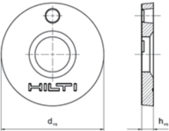
Sealing washer
